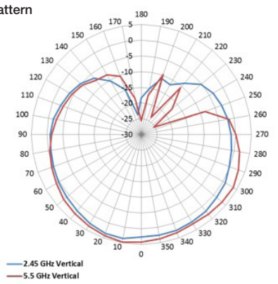
E-Plane Pattern
