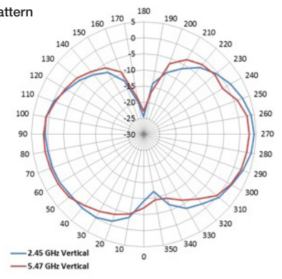
E-Plane Pattern
