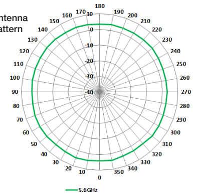
External Antenna E-Plane Pattern
