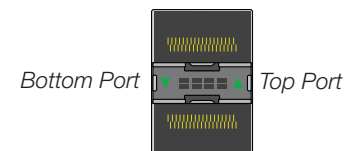
QSFP28 Ports
